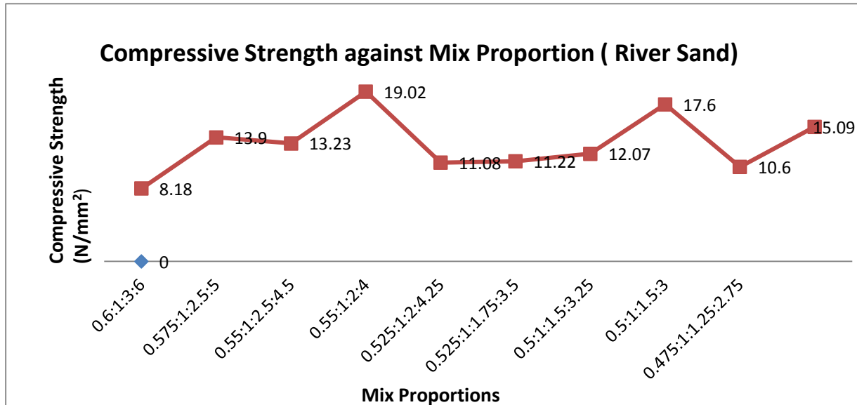
Figure 3 Graph of compressive strength against mix proportion (River Sand)
