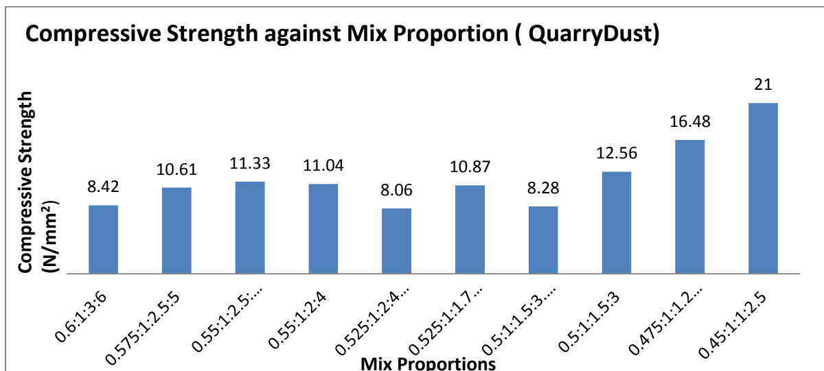
Figure 2 Bar chart showing compressive strength against mix proportion (Quarry Dust)
