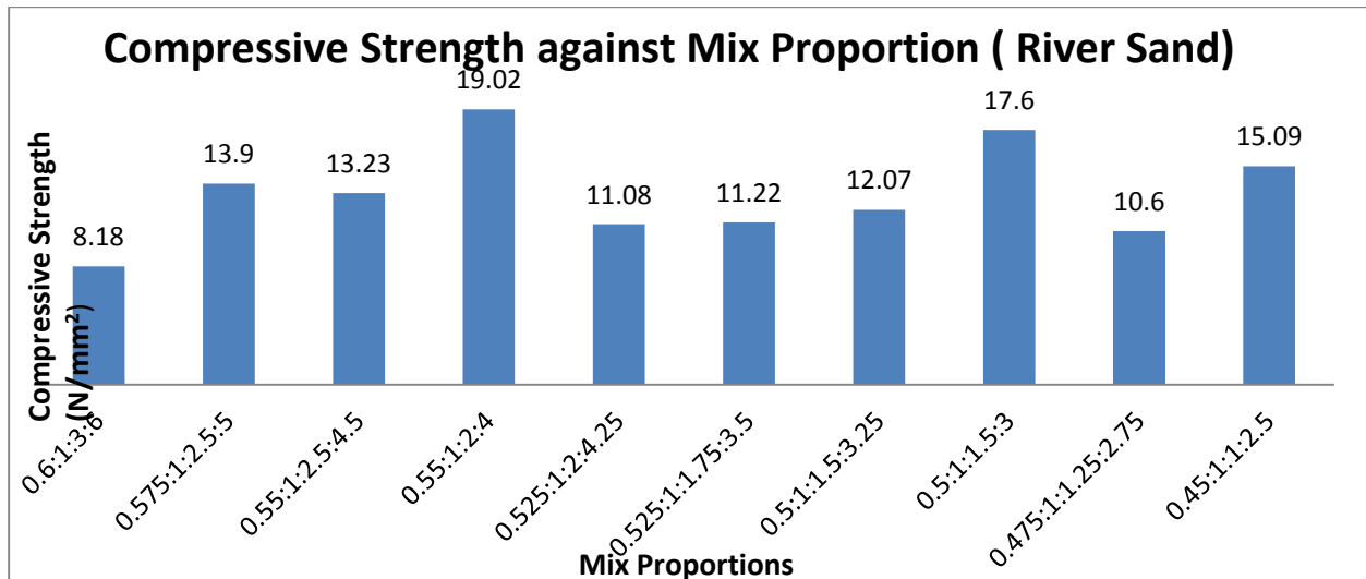
Figure 4 bar chart showing compressive strength against mix proportion (River Sand)
