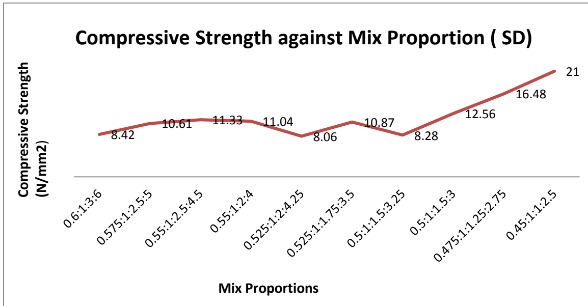
Figure 1 Graph of compressive strength against mix proportion (Quarry Dust)
